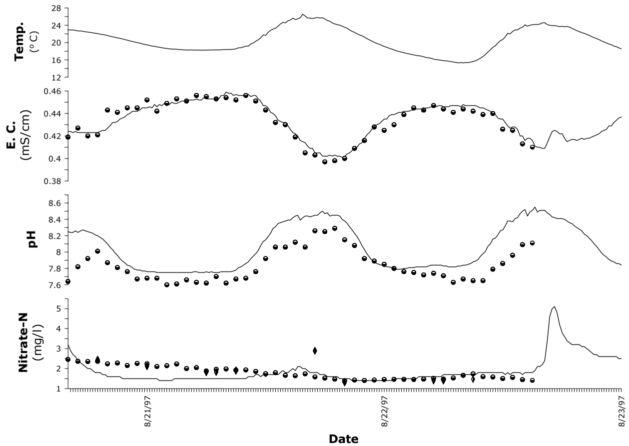
Figure 4. Comparison of YSI Data to Hourly Grab Data.
