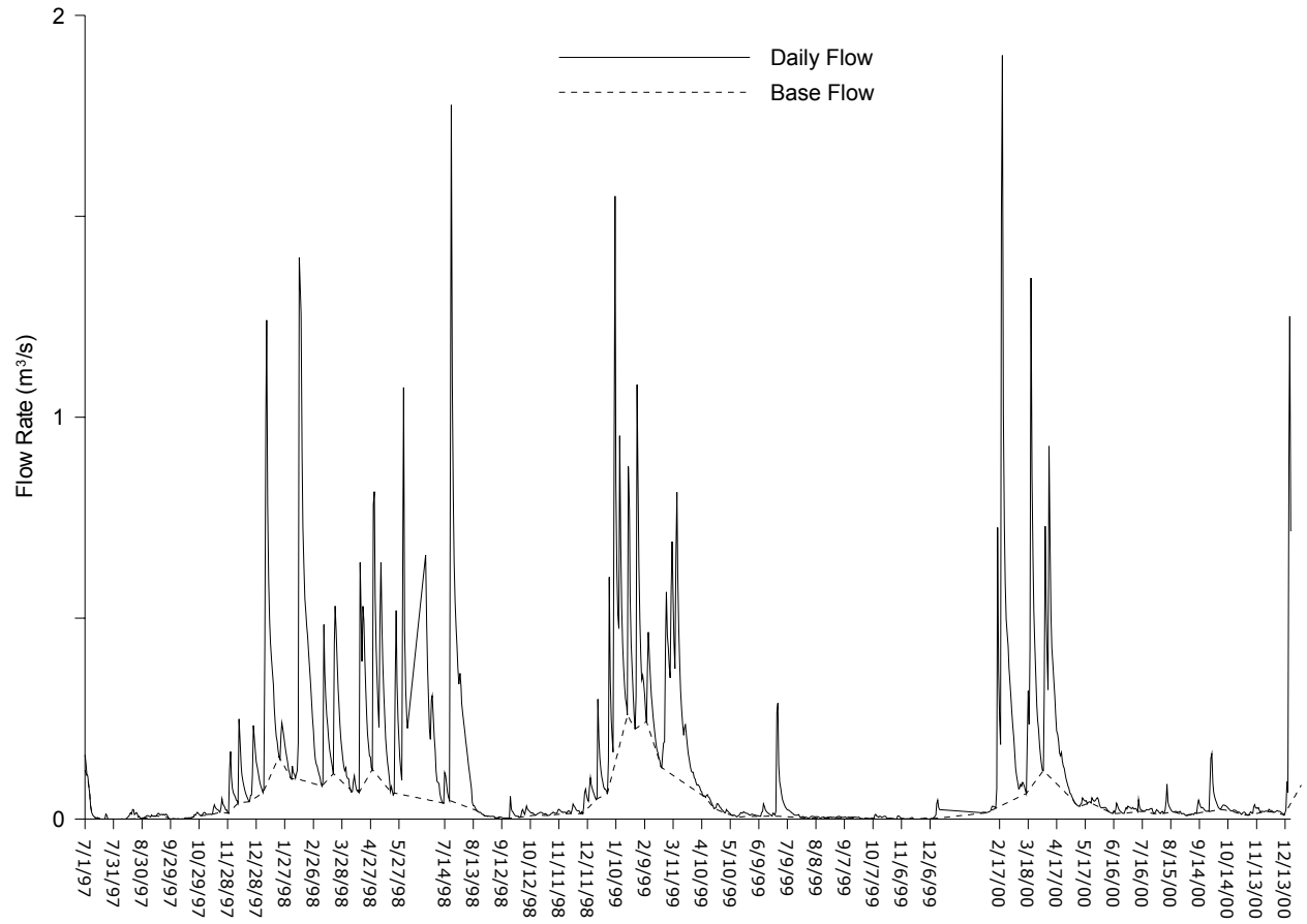
Figure 3. Mean Daily Flow and Mean Daily Baseflow at the UKARC Pour Point.
